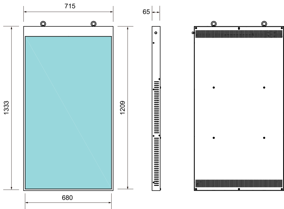
Outline drawing of standard module, (mm)
