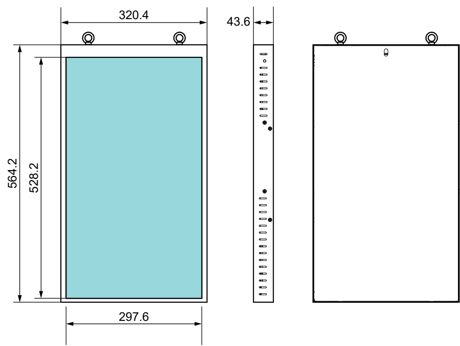
Outline drawing of standard module, (mm)
